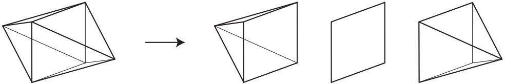
Figure 6 The interior faces of a matroid subdivision of the uniform matroid U_{2,4} .
