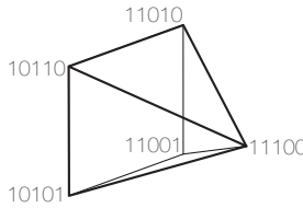
Figure 3 The matroid polytope for the matroid (2.1). The vertices correspond to the bases.
